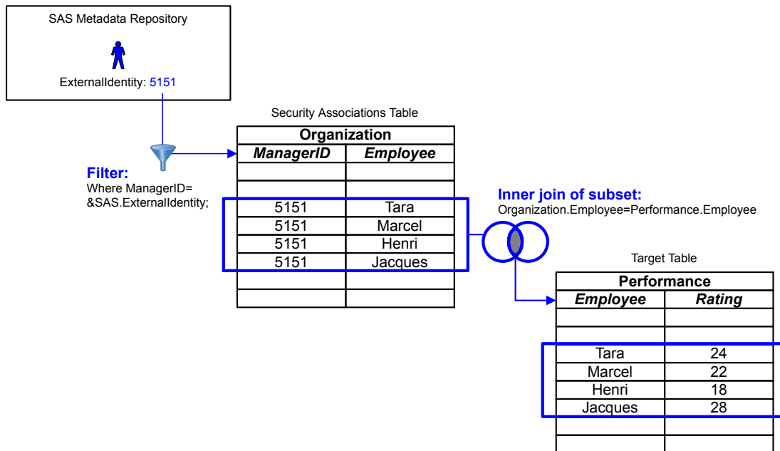
Figure 5.3 Performance Example: Data Model
