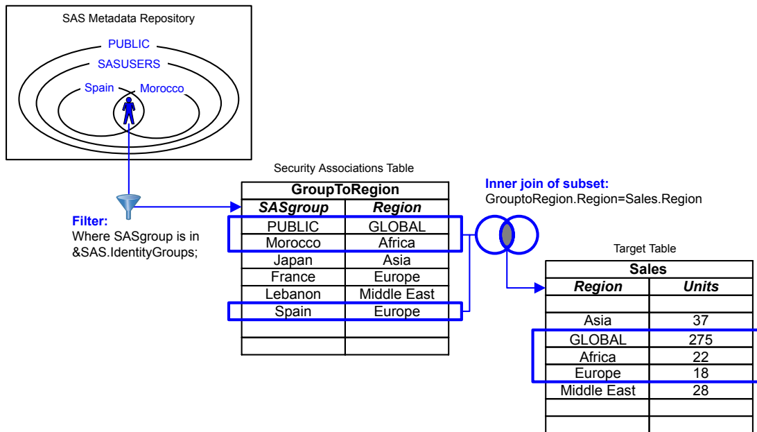
Figure 5.4 Sales Example: Data Model
