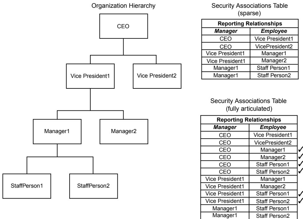
Figure 5.5 Representations of an Organizational Hierarchy
